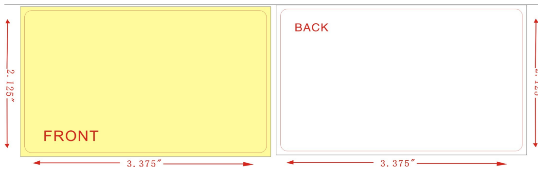
(PVC) Magnetic card with Hanger 3.375"x 7.125"
